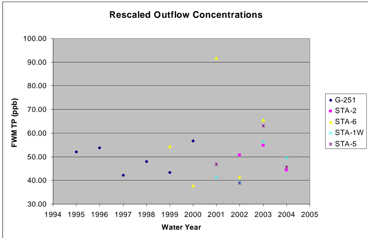
Figure 2 – Annual FWM phosphorus concentrations at STA outflow structures, rescaled to 50 ppb.
